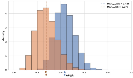
Fig. 1. Histogram of AP@k values for Scenario A3 ( N = 50, m = 25, p = 0.5, k = 40 ). The SWOR distribution (blue) is shifted to higher values compared to SWR (orange), reflecting normalization by \min(m, k) in the offline case.
