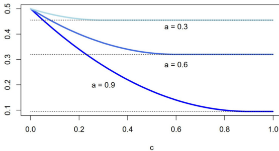
Fig. 3. The upper bound on the right-hand side drawn as a function of c for some chosen values of a . The dotted lines show the value (1 - a^2)/2 for each a
