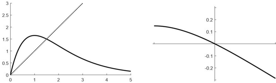
Fig. 4. The function f(x) = xe^{r-x} for r = 1.5 . We have a fixed point at x = r . On the right, we see a part of the plot with the fixed point moved to the origin
