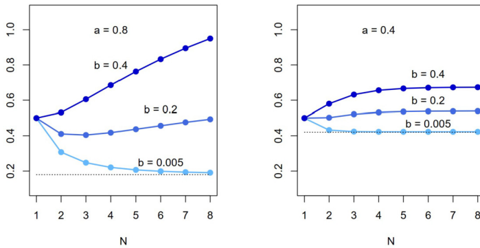
Fig. 2. The upper bound on the right-hand side illustrated for different values of a and b and N = 1 (when the value is 1/2 ) and N = 2, \dots, 8 . The dotted line shows the value (1 - a^2)/2 in each case
